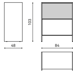
LN 10302 sideboard 84x48x103 madia 84x48x103 placard 84x48x103
