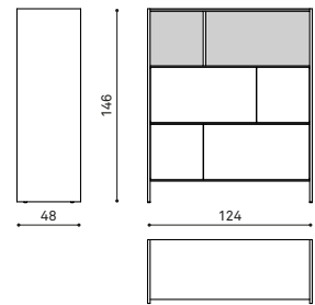
LN 14602 sideboard 124x48x146 madia 124x48x146 placard 124x48x146
