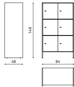
LN 14601 locker 84x48x146 locker 84x48x146 casiers 84x48x146
