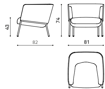
SH 7090 armchair 81x82x74 poltrona 81x82x74 fauteuil 81x82x74
