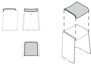
NM 100C NM 1000 stool cushion Cuscino per sgabello NM 1000 Coussin de tabouret NM 1000
