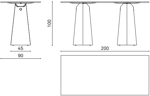
NM 200100 Table 200x90, h 100 Tavolo 200x90, h 100 Table 200x90, 100
