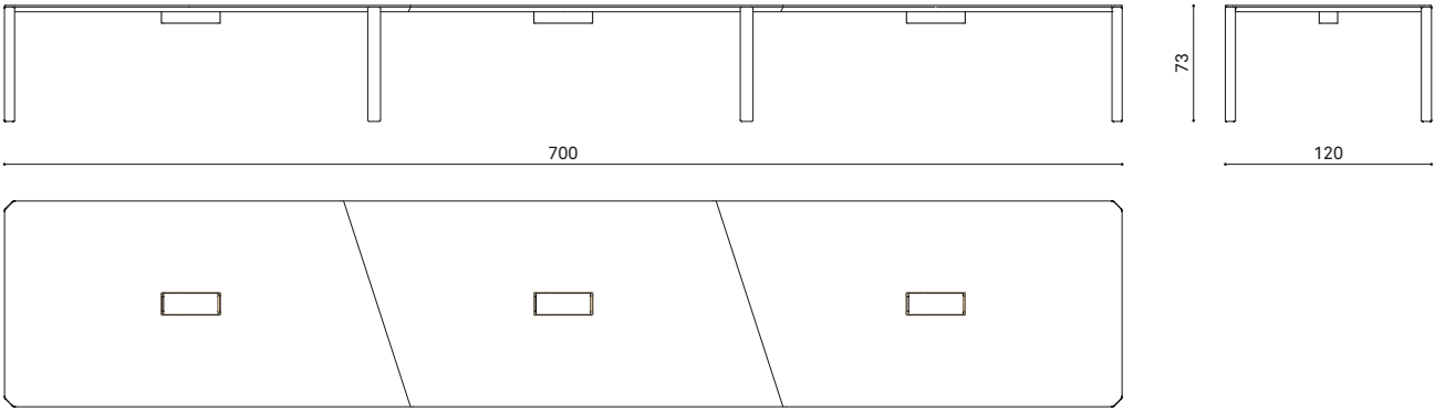
ERB 700120 table 700x120cm tavolo 700x120cm table 700x120cm
