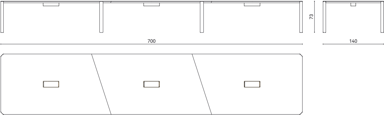
ERB 700140 table 700x140cm tavolo 700x140cm table 700x140cm
